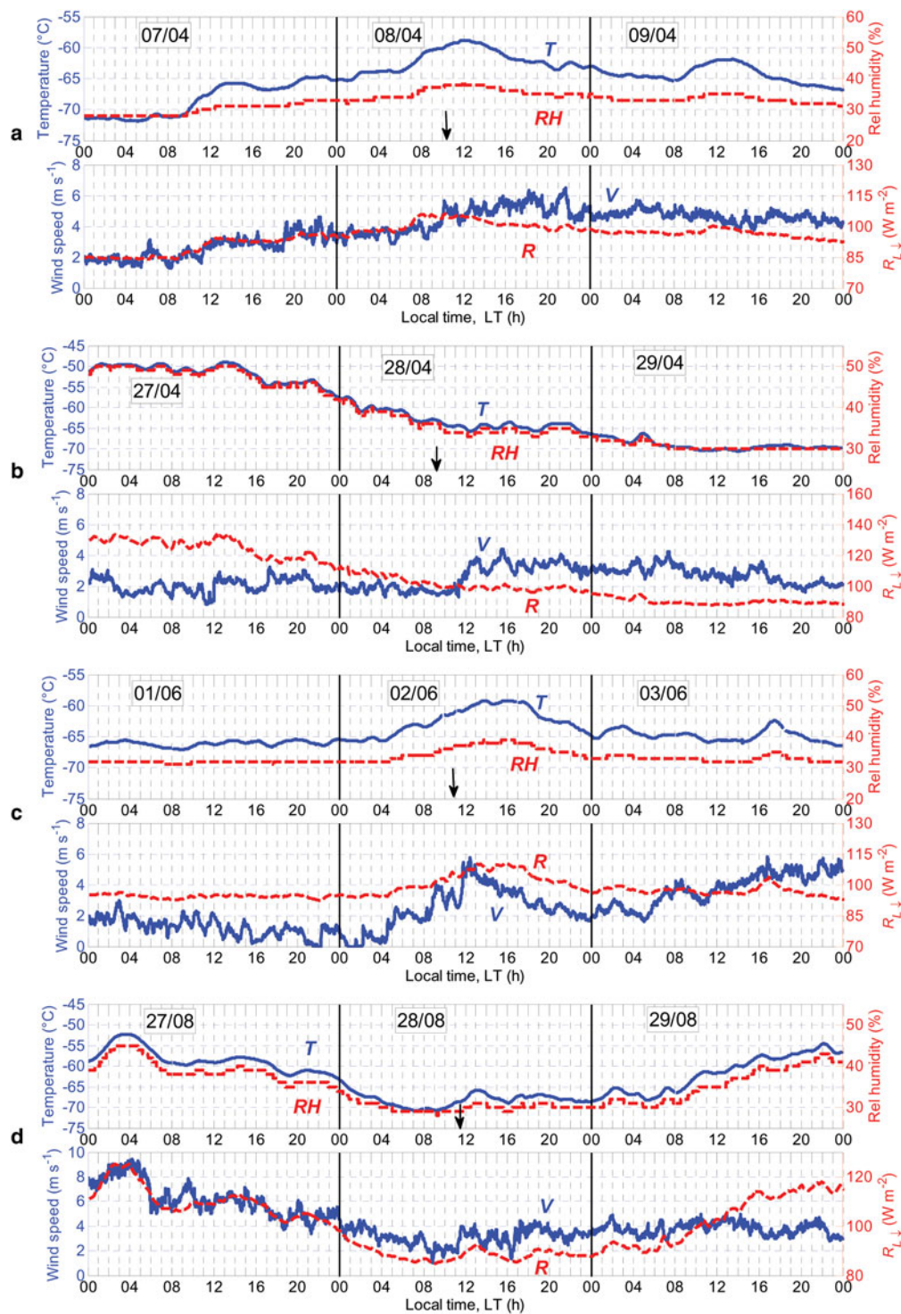
Fig. 2. Time behaviour of meteorological parameters. a 07–09 April 2014 b 27–29 April 2014 c 01–03 June 2014 d 27–29 August 2014 Date format on plots is dd/mm. The top panels display temperature T (blue solid curve) and relative humidity RH (red dash curve). The bottom panels display wind speed V (blue solid curve) and longwave downward radiation R_{L\downarrow} (red dash curve). Black arrows indicate the times after which yukimarimo were observed.
