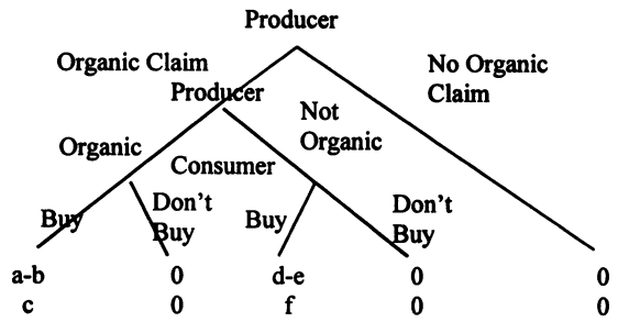
Figure 1. Search Good
