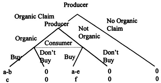
Figure 2. Experience Good
