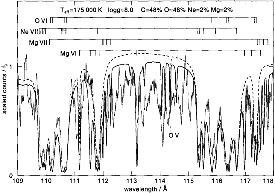
Figure 3. Detail from the Chandra count spectrum of H 1504+65 (thin line), shifted by -0.06 \text{ \AA} to zero radial velocity. Relative fluxes of two models are overplotted, one including Mg (solid line) and one without Mg (dashed line), in order to facilitate the identification of Mg lines. Observation and model spectra are smoothed with Gaussians (FWHM 0.02 \text{ \AA} and 0.03 \text{ \AA} , respectively).
