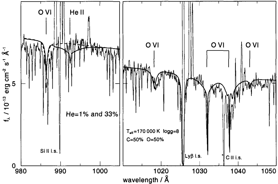
Figure 1. Details from the FUSE spectrum of H 1504+65. Left panel: The lack of the He II ( n = 2 \rightarrow 7 ) absorption line confirms the He-deficiency. Overplotted are two models with 33% He and 1% He. Right panel: The O VI resonance doublet shows no signature of a stellar wind. Narrow absorption lines are of interstellar origin (mostly H 2 ) and emission lines are from the geocorona. All spectra are smoothed with Gaussians (0.1 \text{\AA} FWHM).
