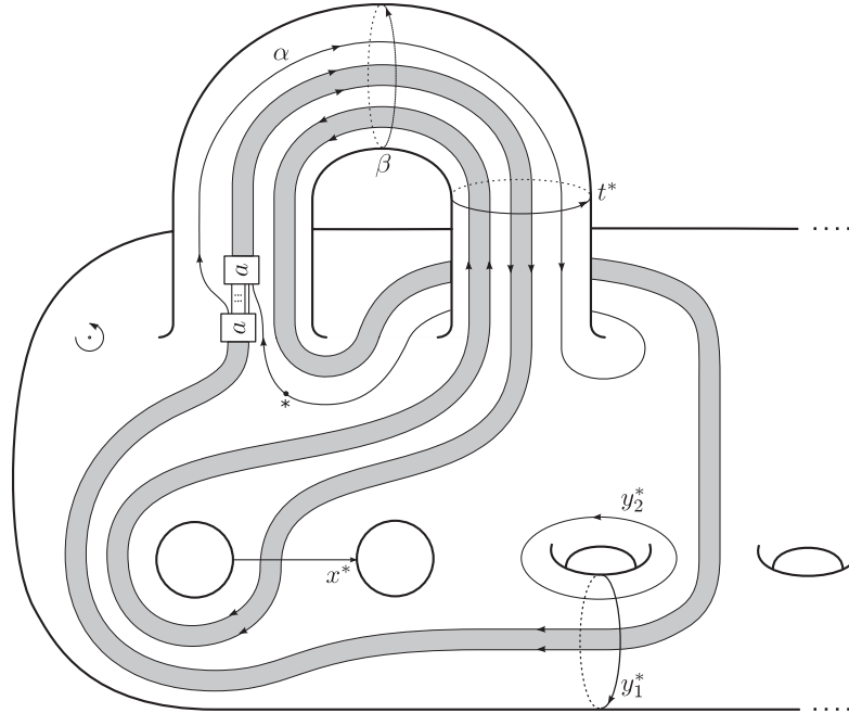
FIGURE 1. Attaching circle \alpha on \Sigma_1 .
