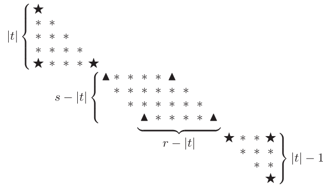
FIGURE 3. Support of \tau(M(r, s, t)) .
