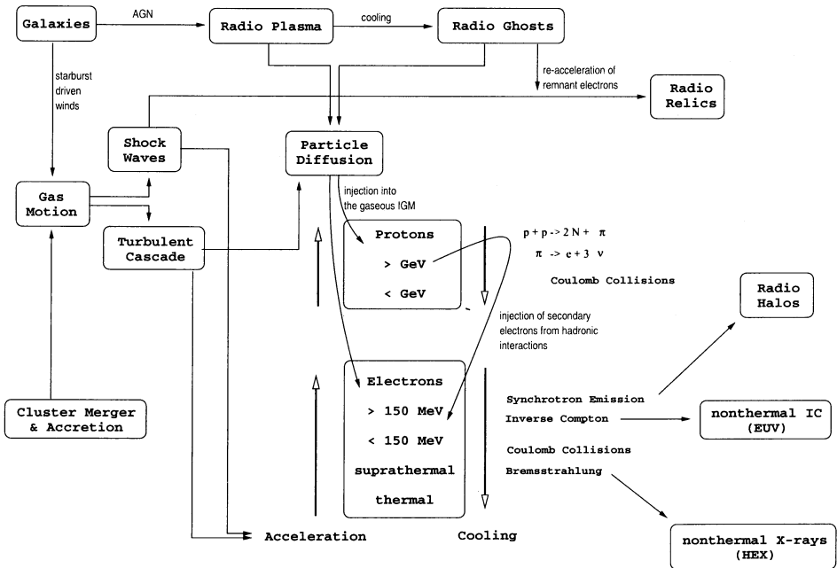
Figure 1. Network of processes possibly responsible for non-thermal cluster emission. Description in the text.
