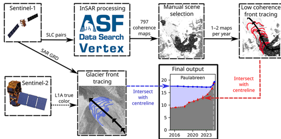
Figure 2. Conceptual diagram of the acquisition and processing of the data. The data examples are from Paulabreen (Figure 4e–h) and showcase the delineation of the lower low-coherence boundary (red) and terminus positions (blue) for its plot in Figure 5e (see that caption for a further explanation of the plot). For up-glacier propagating low-coherence fronts, there is an additional step (green lines, e.g. in Figure 1) to delineate the upper boundary. The latter date in the acquisition pair for the exemplified coherence map ('Manual scene selection' box) is 1 April 2020, and the SAR backscatter image ('Glacier front tracing' box) date is 24 December 2024.
