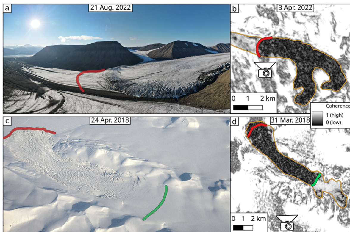
Figure 1. Photographs compared to coherence maps in the same year. (a) Down-glacier propagating surge of Vallåkrabreen, showing a surge bulge with splaying crevasses and a less pronounced forebulge ahead of it (photograph credit: Leonard Magerl). The red line shows the approximate location of the low-coherence boundary from earlier that year (shown in (b)), together with the photo location; roughly coincident with the forebulge. (c) Up-glacier propagating surge of Arnesenbreen (photograph credit: Erik S. Mannerfelt), showing the lower surge boundary in red and the upper low-coherence boundary in green (cf. panel (d)). We presume that the discrepancy between the green line in (c) and the region of substantial crevassing is due to coherence being sensitive to smaller disturbances than what can be seen in a winter photograph. The largest surge extent (so far) is shown in yellow outlines for panels (b) and (d). The dates of the coherence maps represent the latter dates of the acquisition pairs. Areas outside the largest surge extents have reduced contrast to enhance visibility.
