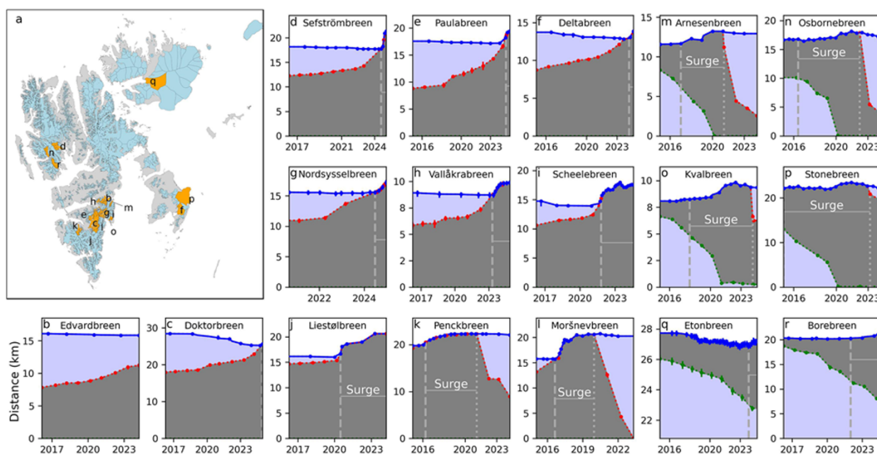
Figure 5. Digitised low-coherence (surge) front and terminus progressions for surges on Svalbard: lower low-coherence boundary/surge-front (red); terminus (blue) and upper low coherence boundary (green). See Figure 2 for the method. (a) Overview map showing all glaciers (light blue) and the location of the presented glaciers (orange plus letters). Glacier front outlines are from Nuth and others (2013). (b) Low-coherence front progression that indicates a potential future advance. (c–l) Down-glacier (bulge) propagating surge examples. (m–r) Up-glacier (terminus initiated) propagating surge examples. The y-axis represents the total distance along the centreline from the top of the glacier. High-coherence parts of the glacier are shaded light blue, low-coherence parts are shaded grey. Points (with 25th to 75th percentile spreads) represent measured values, and the parts in between are interpolated. For reference, (c) is lake-terminating, (h, i) (before reaching the sea in 2022) and (k) are land-terminating, and the rest are tidewater glaciers.
