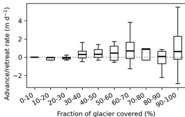
Figure 3. Boxplot comparison of the fraction of low coherence and terminus fluctuation rate at up-glacier propagating (terminus initiated) surges. This was used to derive the 40% threshold as a common starting point for these surges; the 40–50% bin is the first and only bin where the first quartile (the lower box boundary) is above 0 m d -1 .
