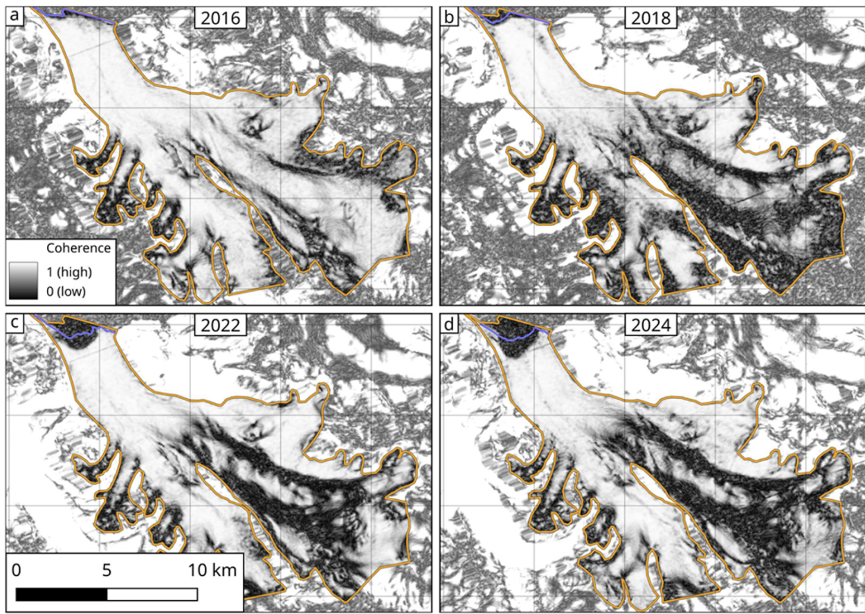
Figure 6. Early surge bulge detection at Kongsvegen, observed visually through changes in InSAR coherence maps. The 5 \times 5 km grid cells show that little progression is observed, but shear margins along the bulge show a progressive reduction in coherence. The yellow outlines in all panels represent the maximum extent of the glacier throughout the study period (2016–), and the blue lines represent the concomitant front positions. The dates for the latter SAR acquisition in the coherence maps are (a) 10 April, (b) 19 March, (c) 3 April and (d) 23 March. Areas outside the largest surge extents have reduced contrast to enhance visibility.
