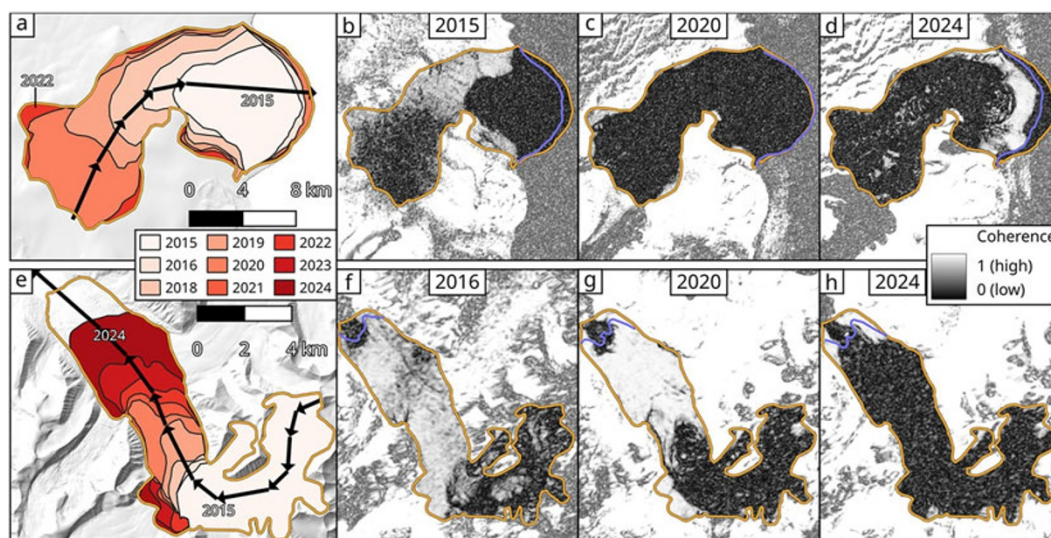
Figure 4. Examples of coherence changes during the progression of two surges. Top (a–d): terminus-initiated surge of Stonebreen. Note the onset of stagnation in 2024 (d) shown by the terminus regaining coherence. Bottom (e–h): surge bulge propagation of Paulabreen. The dates for the latter SAR acquisition in the coherence maps are (b) 21 January, (c) 3 March, (d) 22 March, (f) 29 March, (g) 1 April and (h) 23 March. The yellow outlines in all panels represent the maximum attained extent of the surges so far, and the blue lines represent the concomitant front positions. Basemap hillshade from 2010 of panels (a) and (e) courtesy of the Norwegian Polar Institute (2014). Areas outside the largest surge extents have reduced contrast to enhance visibility.
