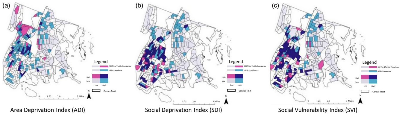
Figure 2. Choropleth maps.
