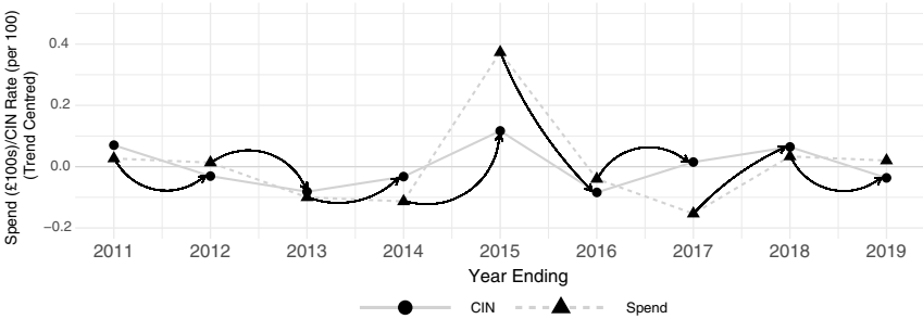
FIGURE 2. A visual explanation of the effects of removing variance associated with case intercepts and slopes on the interpretation of lagged effects
