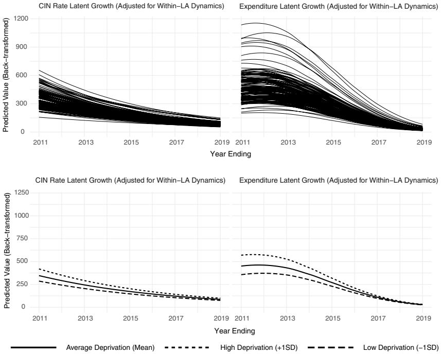
FIGURE 3. Predicted trajectories over time from latent growth variables in ALT-SR model
