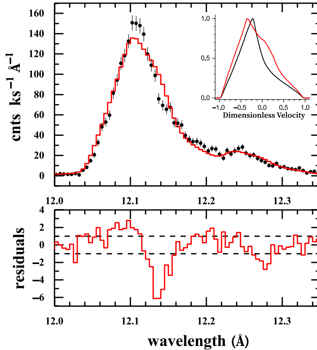
Figure 2. Same as Figure 1 except this panel illustrates a simulation of the precision we expect for the spectrum using the full approved Cycle 19 Chandra exposure time. This will greatly enhance our ability to differentiate models as evident in the clear trends which are apparent in the simulated residuals. The inset shows the theoretical line shapes for the smooth wind (black) and clumped (red) models before the inclusion of any instrumental effects. The normalized theoretical line profile models in the inset are displayed as a function of the dimensionless velocity (i.e. the line-of-sight wind velocity divided by the terminal velocity, with 0 representing the rest wavelength for the line). This calculation assumes a value of 2250 \text{ km s}^{-1} for the terminal velocity (Puls et al. 2006).
