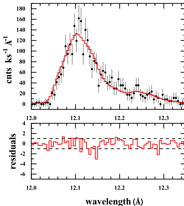
Figure 1. Comparison of the MEG Ne X region clump model (solid line) to a simulated smooth wind dataset with errors appropriate to the existing 2000 HETG observation. The large errors per bin make it difficult to make precise determinations of the model parameters, and there is no clear pattern in the residuals. The residuals are in the sense of (model) minus (simulated model) divided by the simulated error for each bin. This diagram is constructed using the standard bin size for the MEG detector ( 0.005 \text{ \AA} ).
