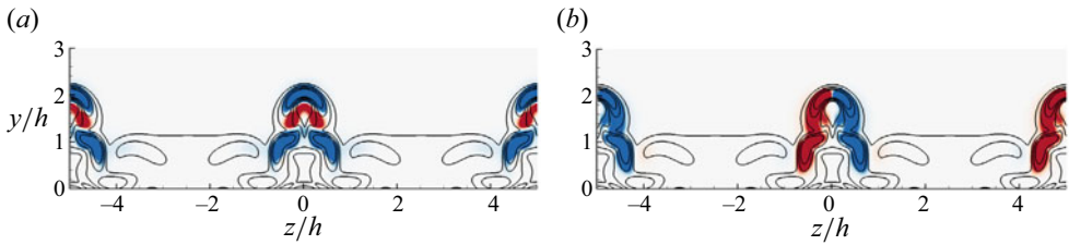
Figure 17. Contour plots of P_y = -|\hat{u}||\hat{v}|\partial\bar{u}/\partial y (a) and P_z = -|\hat{u}||\hat{w}|\partial\bar{u}/\partial z (b) in the cross-flow plane of x = 12.5h for case (5h, 5h) at Re_h = 600 . The contour levels depict \pm 10\% of the maximum P_y and P_z . The localized shear is depicted by the solid lines of u_s = ((\partial\bar{u}/\partial y)^2 + (\partial\bar{u}/\partial z)^2)^{1/2} from 0 to 2.
