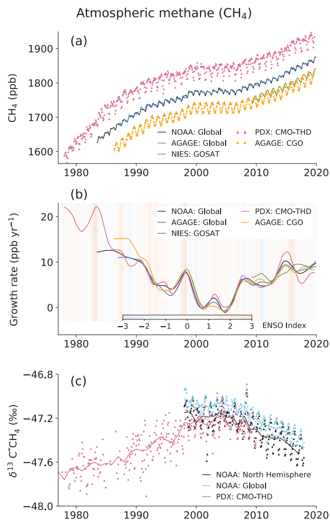
Figure 5.13 | Time series of CH 4 concentrations, growth rates and isotopic composition. (a) CH 4 concentrations; (b) CH 4 growth rates; (c) \delta^{13}\text{-CH}_4 . Data from selected site networks operated by the National Oceanic and Atmospheric Administration (NOAA; Dlugokencky et al., 2003), Advanced Global Atmospheric Gases Experiment (AGAGE; Prinn et al., 2018) and Portland Airport (PDX, Portland State University; Rice et al., 2016). To maintain clarity, data from many other measurement networks are not included here, and all measurements are shown in the World Meteorological Organization X2004ACH 4 global calibration standard. Global mean values of XCH 4 (total-column), retrieved from radiation spectra measured by the Greenhouse Gases Observing Satellite (GOSAT) are shown in panels (a) and (b). Cape Grim Observatory (CGO; 41°S, 145°E) and Trinidad Head (THD; 41°N, 124°W) data are taken from the AGAGE network. NOAA global and northern hemispheric (NH) means for \delta^{13}\text{C} are calculated from 10 and 6 sites, respectively. The PDX data adjusted to NH (period: 1977–2000) are merged with THD (period: 2001–2019) for CH 4 concentration and growth rate analysis, and PDX and NOAA NH means of \delta^{13}\text{C} data are used for joint interpretation of long-term trends analysis. The multivariate El Niño–Southern Oscillation (ENSO) index (MEI) is shown in panel (b). Further details on data sources and processing are available in the chapter data table (Table 5.SM.6).
