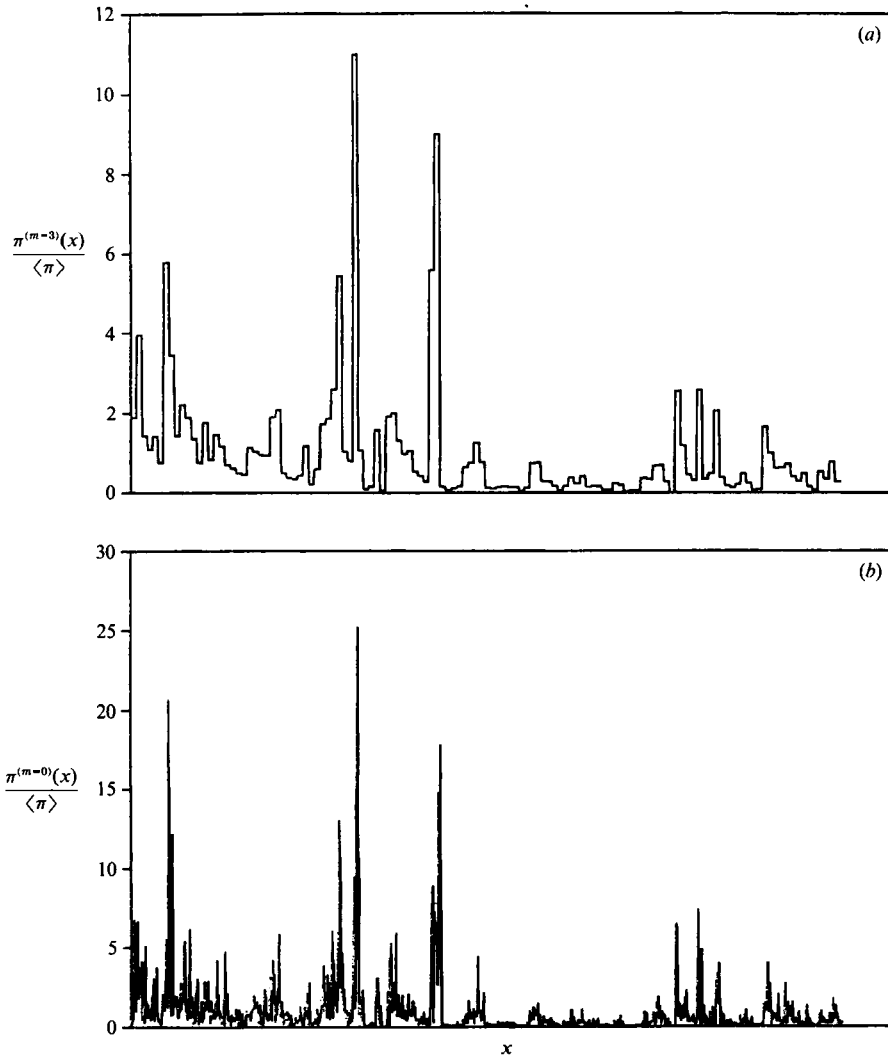
FIGURE 28. Illustration of an intermittent (multifractal) field generated by a multiplicative process in one dimension. The horizontal axis is successively divided into smaller halves, and the area under the curve is multiplied by a random multiplier \xi . The distribution of multipliers \xi is a triangular one (see text), (a) is the result after such a process after 7 iterations, (b) is after 10 iterations. Notice that such fields are positive everywhere.
