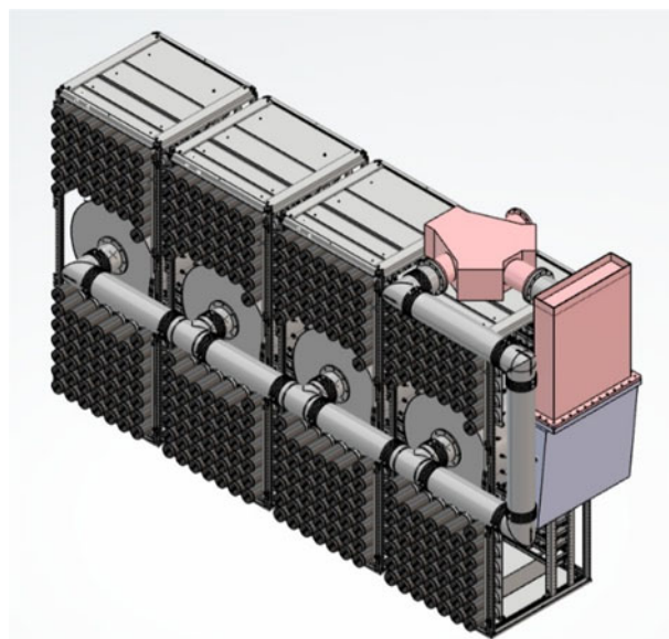
Figure 2. 3D view of the solid state power amplifier station at 400 kW.
