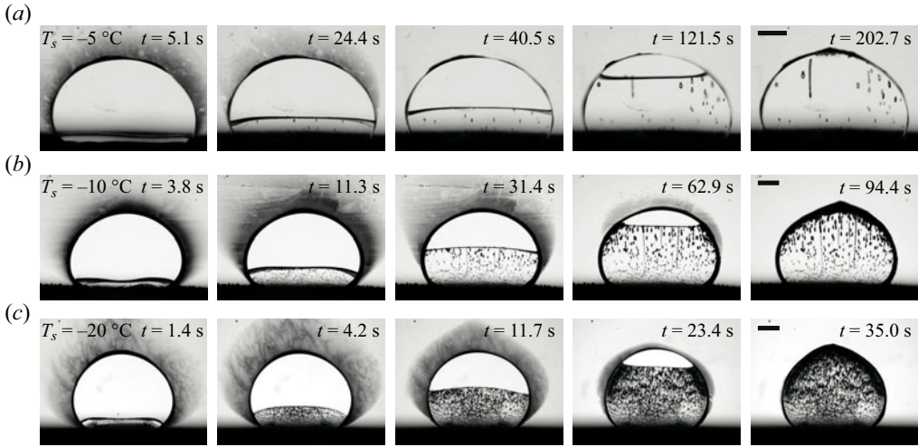
Figure 2. Sequences of images (supplementary movies 1–3 available at https://doi.org/10.1017/jfm.2024.777 ) highlighting the differences when freezing a sessile drop of equal volume ( V_d = 25\text{ }\mu\text{l} ) sandwiched between two acrylic plates at three different substrate temperatures, i.e. (a) T_s = -5\text{ }^\circ\text{C} , (b) T_s = -10\text{ }^\circ\text{C} , and (c) T_s = -20\text{ }^\circ\text{C} from top to bottom, respectively. All scale bars (right panels) are 1 mm.
