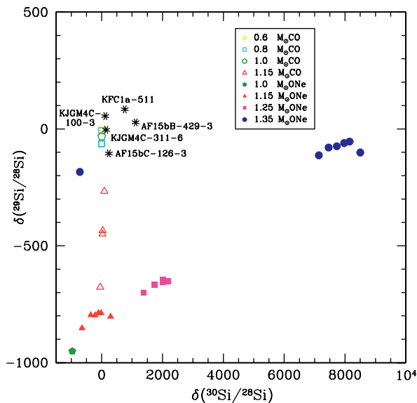
Figure 4 Same as Fig. 1, for silicon isotopic ratios, expressed as delta values (deviations from the solar Si isotopic ratios in permil).
