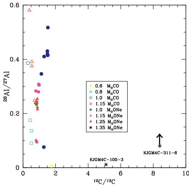
Figure 3 Same as Fig. 1, for aluminium versus carbon isotopic ratios.
