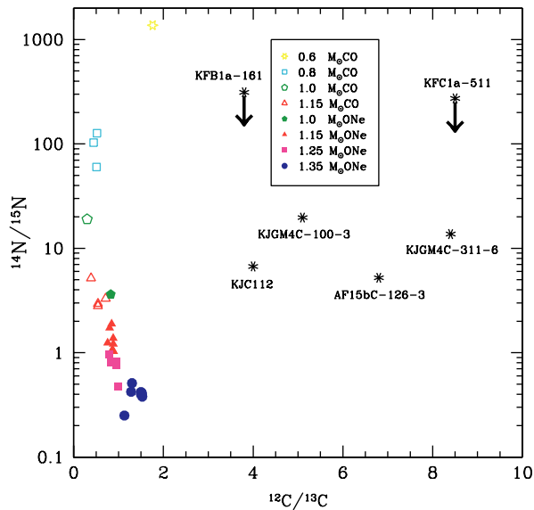
Figure 1 Nitrogen versus carbon isotopic ratios, obtained from a series of hydrodynamic models for both CO and ONe novae (José & Hernanz 1998; Hernanz et al. 1999; José et al. 1999, 2001; and unpublished data). Data from presolar nova grains isolated from the Acfer 094 and Murchison meteorites (Amari et al. 2001; Amari 2002) are also shown.
