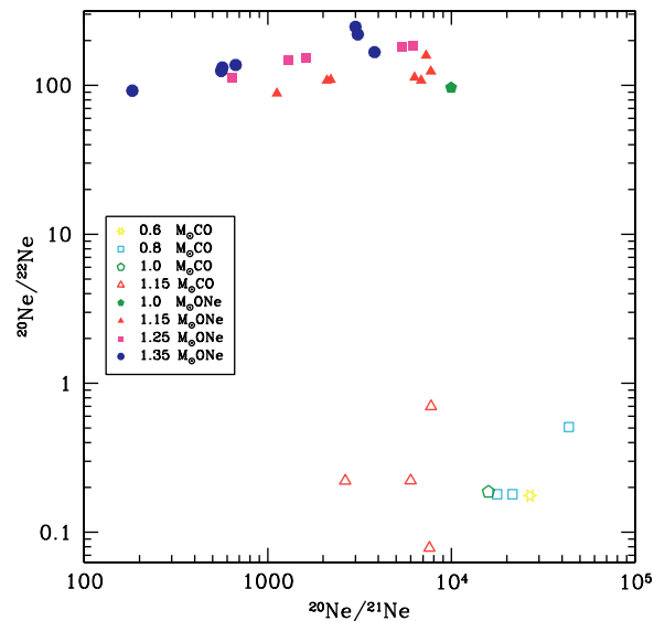
Figure 2 Same as Fig. 1, for the ^{20}\text{Ne}/^{21}\text{Ne} and ^{20}\text{Ne}/^{22}\text{Ne} isotopic ratios. An upper limit of ^{20}\text{Ne}/^{22}\text{Ne} < 0.01 has been determined for graphite grain KFC1a-161 (see Nichols et al. 2003).
