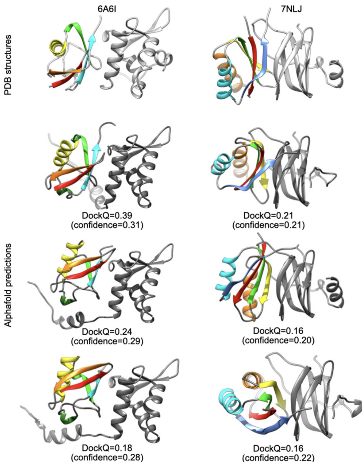
Fig. 2. Comparison between PDB structures and AlphaFold2 predictions for 6A6I and 7NLJ.
