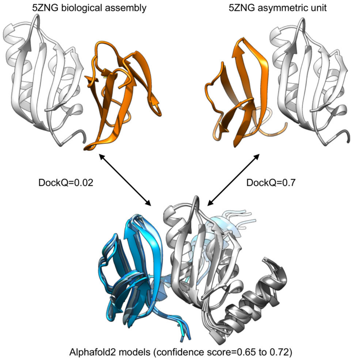
Fig. 1. Comparison between the structural information available for 5ZNG and the AlphaFold2 models. The biological assembly discussed in the article introducing the structure is the one annotated as asymmetric unit in the PDB (top right).
