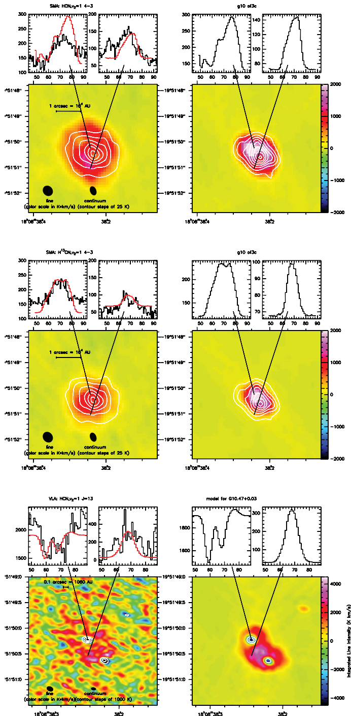
Figure 2. radmc-3d model (right) of observed lines (left) of vibrationally excited HCN(4–3) (top), H 13 CN(4–3) (center), and the J = 13 \ell -type line of HCN in G10.47.
