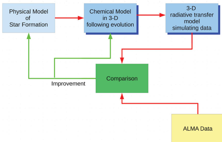
Figure 1. Scheme for modeling ALMA data. To minimize the number of free parameters, it is best to start from physical and chemical models, which then may have to be modified based on the comparison. The comparison itself needs to be done automatically, in a fashion that gives not only the best fit solution, but also information about the quality of the fit, the existence or not of secondary minima, and confidence intervals of parameters.
