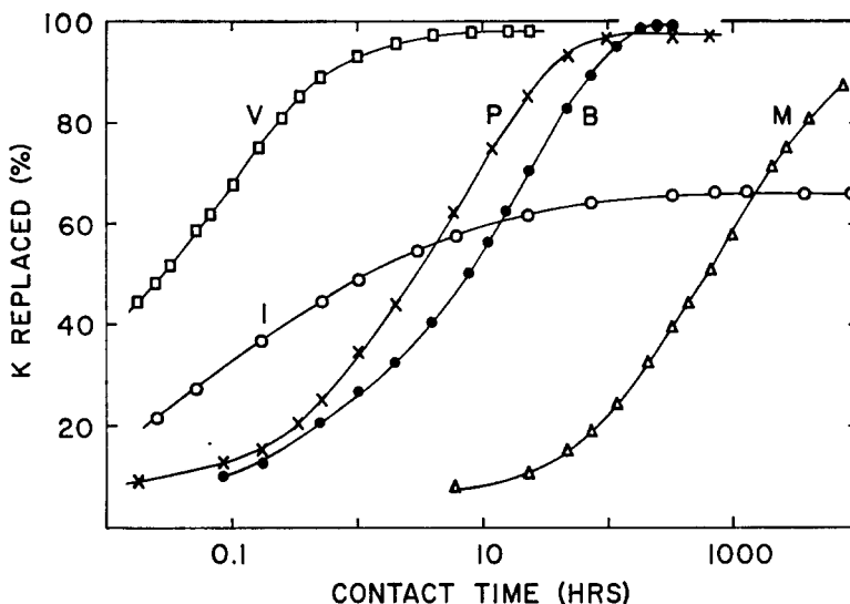
FIG. 4. K extracted from < 2 \mu illite and < 50 \mu vermiculite, phlogopite, biotite and muscovite samples in NaCl-NaTPB solutions.
