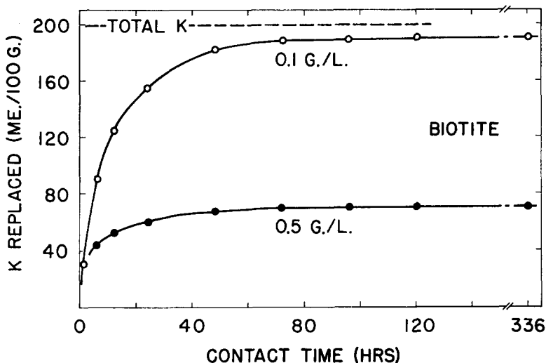
FIG. 1.—K extracted by equilibrating 0.1 and 0.5 g samples of 10–20 \mu biotite in 1 liter 1 N NaCl.
