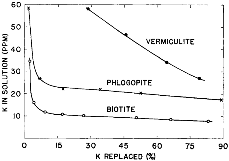
FIG. 2.—Relationship between the equilibrium levels of K in 1 N NaCl solutions and the amounts of K extracted from 10–20 \mu samples of biotite, phlogopite and vermiculite.
