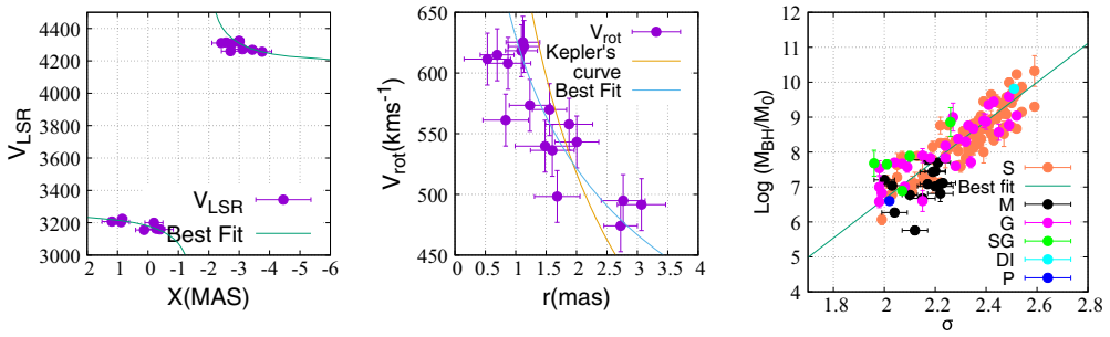
Figure 1. (left) Plot for line-of-sight velocities for blue-shifted and red-shifted maser features of NGC3393 (as an example), (middle) Keplerian and Non-Keplerian rotation curves for NGC3393, and (right) The Maggorian Relationship due to the stellar dynamical modelling [S], megamaser technique [M], gas dynamical modelling [G], stellar gas dynamical modelling [SG], direct imaging [DI], and due to the proper motion [P]
