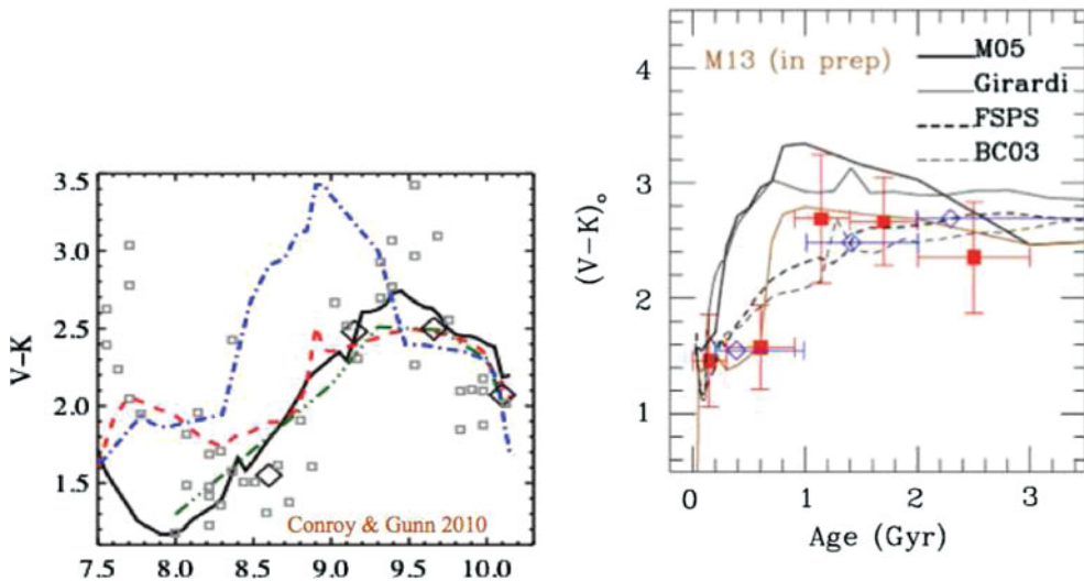
Figure 4. Left-hand panel. Re-calibration of the TP-AGB for SP models by Conroy & Gunn (2010), using the V - K colour of stellar population models as indicator. Plotted towards their revised age scale, the M05 models (blue line) appear mis-calibrated. The BC03 models are shown as red lines. Large diamonds are averages of Magellanic Clouds GCs data. Right-hand panel. Re-calibration of the Conroy & Gunn's re-calibration by Noëll et al. (2013). The early results of M98, namely the onset of the TP-AGB as a sharp transition around 1 Gyr of age, are confirmed.
