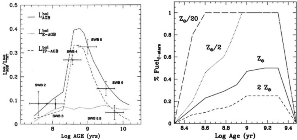
Figure 2. Left-hand panel. From M98: Calibration of the bolometric contribution of the TP-AGB phase for SP models (lines) with star clusters data (symbols with errors). Right-hand panel From M05: Dependence of metallicity on the TP-AGB fuel consumption.
