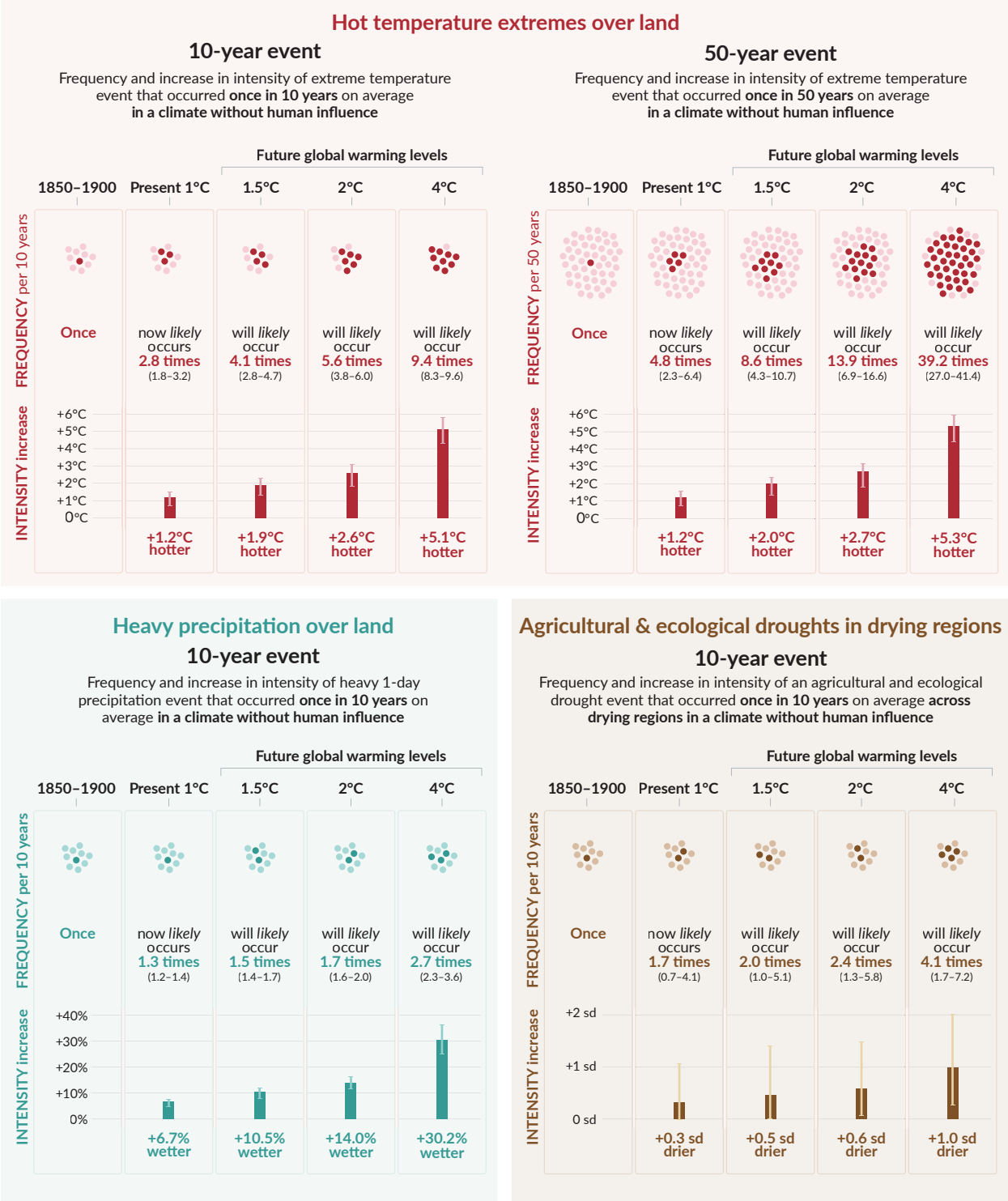
Figure SPM.6 | Projected changes in the intensity and frequency of hot temperature extremes over land, extreme precipitation over land, and agricultural and ecological droughts in drying regions Projected changes are shown at global warming levels of 1°C, 1.5°C, 2°C, and 4°C and are relative to 1850–1900, 9 representing a climate without human influence. The figure depicts frequencies and increases in intensity of 10- or 50-year extreme events from the base period (1850–1900) under different global warming levels. Hot temperature extremes are defined as the daily maximum temperatures over land that were exceeded on average once in a decade (10-year event) or once in 50 years (50-year event) during the 1850–1900 reference period. Extreme precipitation events are defined as the daily precipitation amount over land that
