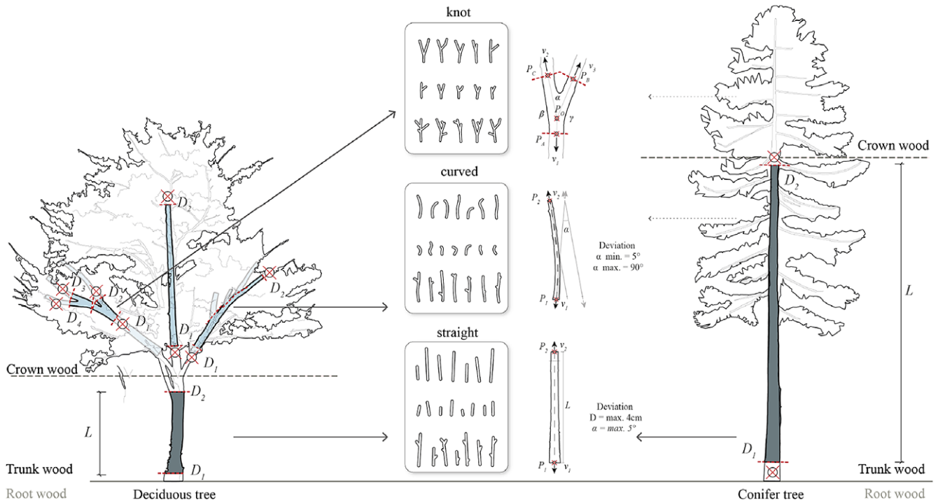
Figure 2. Segmentation of trees and their use for building materials: Straight segments, additionally curved elements and bifurcated elements (knots) (Wages, 2022).
