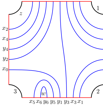
Figure 9. A genus-one Heegaard diagram for (V, Q) .
