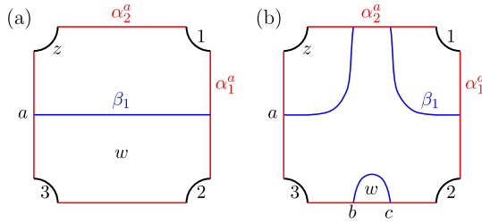
Figure 3. Doubly pointed bordered Heegaard diagrams for the knots C (a) and C_{2,1} (b) in the solid torus V . The boundary segments are labeled according to the convention for CFA.
