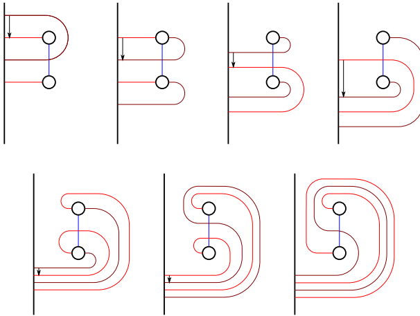
Figure 7. Arc-slide decomposition of T_1 .
