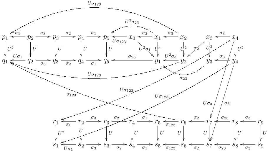
Figure 10. A summand of CFD^-(V, Q_{2,1}) .
