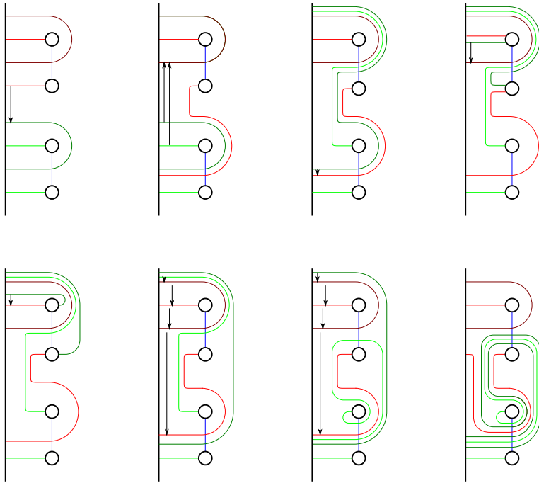
Figure 8. Arc-slide decomposition of T_2 .
