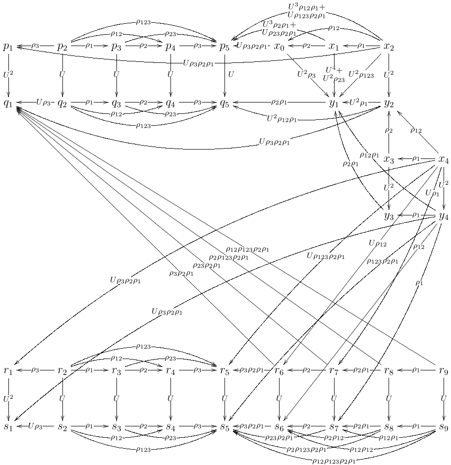
Figure 11. A summand of CFA^-(V, Q_{2,1}) . The only multiplications not shown are the higher multiplications r_i \rightarrow r_j for 5 \leq j < i \leq 9 , which are the same as the ones s_i \rightarrow s_j .
