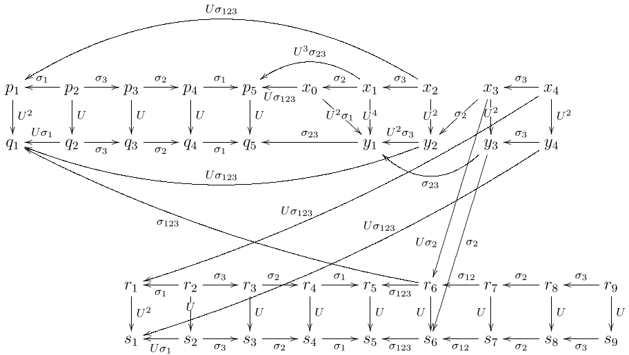
Figure 12. A summand of \text{CFD}^-(V, Q_{2,-1}) .
