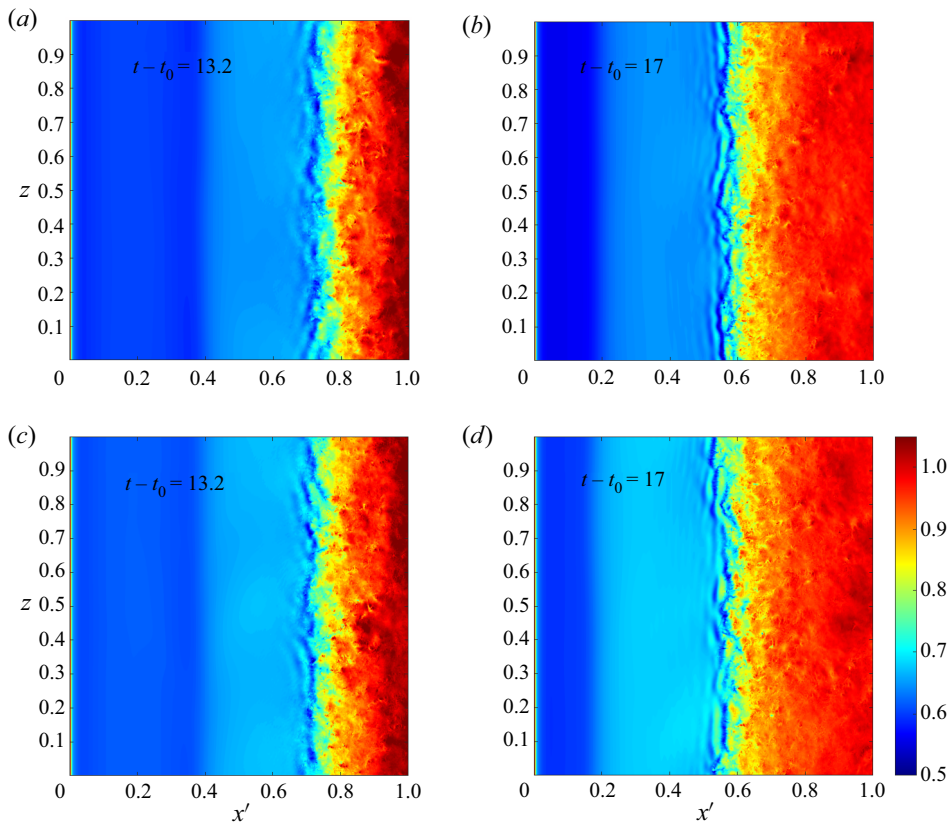
Figure 33. Contours of density on the aerofoil surface shown at (a,c) high- and (b,d) low-lift phases of the buffet cycle for swept cases (a,b) \Lambda = 20^\circ and (c,d) \Lambda = 40^\circ .
