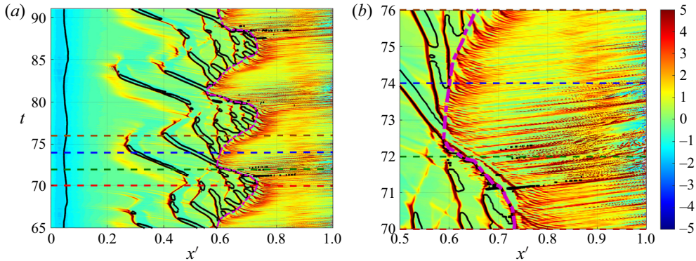
Figure 4. Spatiotemporal variation of streamwise pressure gradient on the suction side of curve C5 for the reference case: (a) entire suction side and (b) close-up. The approximate times associated with different phases of interest, high lift (red), low skin-friction drag (green), low lift (blue) and high skin-friction drag (brown), are highlighted using dashed lines, and the sonic line and the sonic edge (see the text) are shown using solid black and dashed pink curves, respectively.
