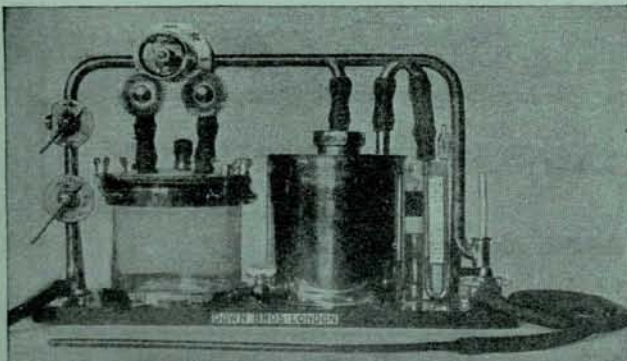
Etherization Apparatus.
