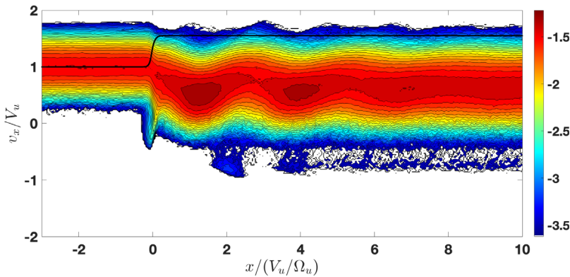
FIGURE 2. The reduced distribution function f(x, v_x) (log scale). The model magnetic field magnitude is shown by the black line.
