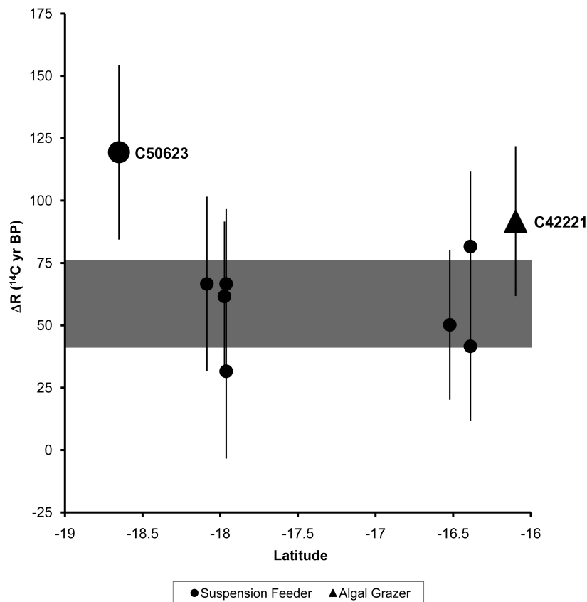
Figure 2 All \Delta R values calculated for this project, excluding F28554 (deposit feeder). Oversized markers indicate values excluded from the regional mean. The gray band indicates the new \Delta R value of 58 \pm 17 ^{14}\text{C} yr recommended as a result of this study.
