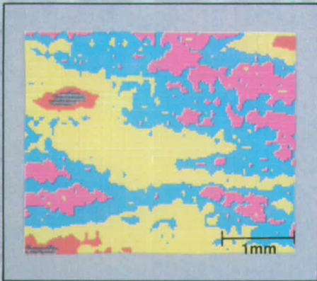
Subgrain Structure
