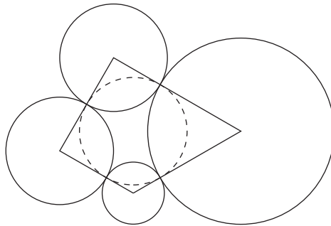
FIGURE 1: A quadrilateral with an inscribed circle
