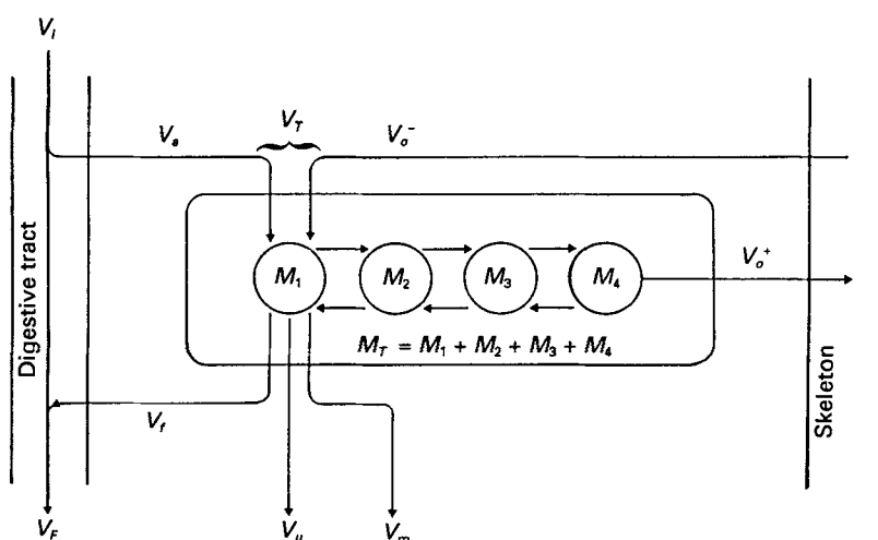
Fig. 2. The model of calcium metabolism. M_1 , M_2 , M_3 and M_4 are compartments of the exchangeable Ca pool M_T . M_1 is the site of tracer administration and is sampled via the blood. Inflows of Ca entering M_1 are from the gut ( V_g ) and bone ( V_o^- ) while outflows from M_1 are losses to milk ( V_m ), urine ( V_u ) and endogenous faecal losses ( V_f ). M_4 is the site of Ca loss ( V_o^+ ) in the non-exchangeable bone, V_i is Ca intake, V_r is Ca transport and V_f is total Ca in faeces.
