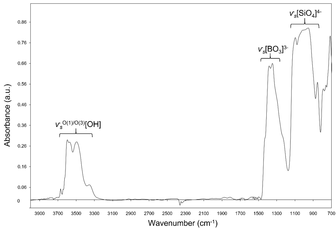
Figure 3. The FTIR spectrum of fluor-rossmanite in the range 4000–700 cm -1 . Bands are observed that are associated with O(1)/O(3) [OH]-stretching modes, [BO 3 ] 3- and [SiO 4 ] 4- stretching and bending modes.
