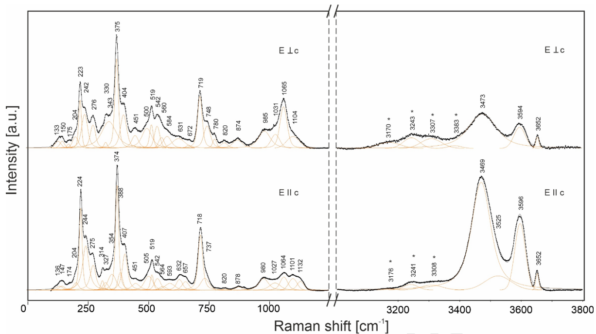
Figure 4. The Raman spectrum of fluor-rossmanite in the range of 80-1250 \text{cm}^{-1} and 3000-3800 \text{cm}^{-1} excited by a 532 nm laser. The upper spectrum corresponds to the orientation of the tourmaline c axis perpendicular to the laser polarization, the lower spectrum corresponds to orientation of the c axis parallel to the laser polarization. The measured spectrum is shown with a dashed line. All observed peaks were fit with Voigt functions and the resultant fit-line (sum) is shown with a solid black line. The luminescence peaks are marked with an asterisk.
