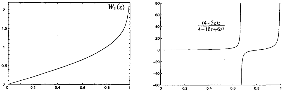
FIGURE 2. Graphs of W_1(z) and (4 - 5z)z / (4 - 10z + 6z^2) .
