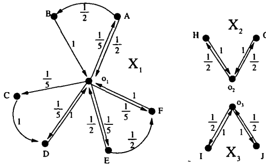
FIGURE 1. Some non-Cayley graphs.
