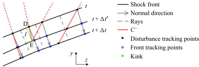
Figure 5. Schematic of the numerical procedure for determining the kink formation on the shock front.
