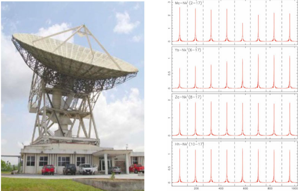
Figure 3. Left: The Kuntunse 32 m satellite communication antenna, Ghana. Right: The first VLBI fringes to the Kuntunse telescope on baselines to the telescopes (top-down) Medicina (Italy), Yebes (Spain), Zelenchukskaya (Russia) and Hartebeesthoek (South Africa).
