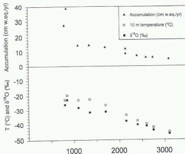
Fig. 4. The 10 m depth temperature ( ^{\circ}\text{C} ), mean \delta^{18}\text{O} (‰) and mean accumulation rate ( \text{cm w.e. a}^{-1} ) at each site vs altitude.
