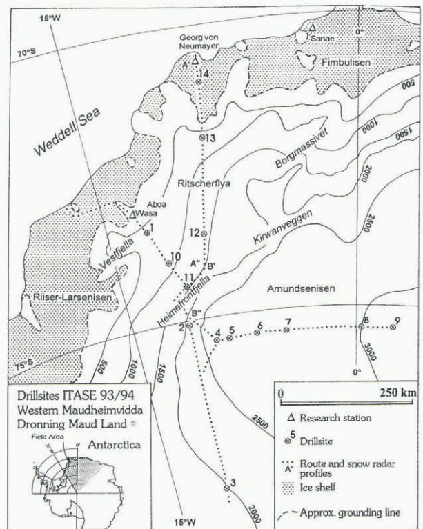
Fig. 1. Map showing locations of the snow pits in western Dronning Maud Land, Antarctica.
