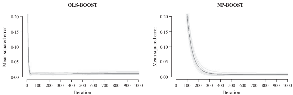
Fig. 3. MSE at each iteration for OLS-BOOST and NP-BOOST in the broiler tuning set in each of the 10 folds (grey line) and the averaged MSE across folds (black solid line). For convenience, only the first 1000 iterations are shown.
