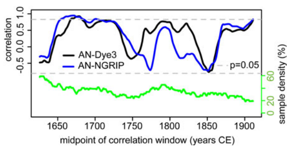
Fig. 4. 50-years running correlation of the ^{10}\text{Be} records of AN versus Dye3 and AN versus NGRIP. The running correlations are shown in black (AN-Dye3) and blue (AN-NGRIP). The sample density (percentage of the 50-year window that was sampled) is shown in green. Local significance levels ( p = 0.05 ) are shown as horizontal dashed line.
