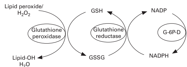
Fig. 1. Conversion of oxidised glutathione (GSSG) to the reduced form (GSH) by glutathione reductase. Glutathione reductase requires riboflavin in the FAD coenzyme form for its activity. G-6P-D, glucose-6-phosphate dehydrogenase.
