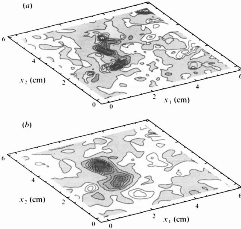
FIGURE 23. Contour plots of SGS energy flux. (a) The flux estimated from the real SGS stress, \Pi_\tau = -\tau_{ij} \tilde{S}_{ij} . (b) The SGS flux implied by the modelled stress \Pi_L = -L_{ij} \tilde{S}_{ij} . Darkest grey corresponds to a maximum value of 0.0288 \text{ m}^2 \text{ s}^{-3} , and the contours are spaced by constant increments of -0.0036 \text{ m}^2 \text{ s}^{-3} . White regions denote negative values.
