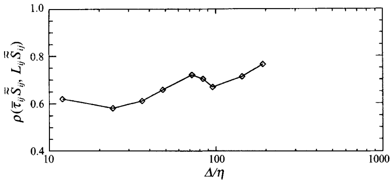
FIGURE 13. Correlation coefficients between L_{pq} \tilde{S}_{pq} and \bar{\tau}_{pq} \tilde{S}_{pq} as a function of \Delta , for the top-hat filter.
