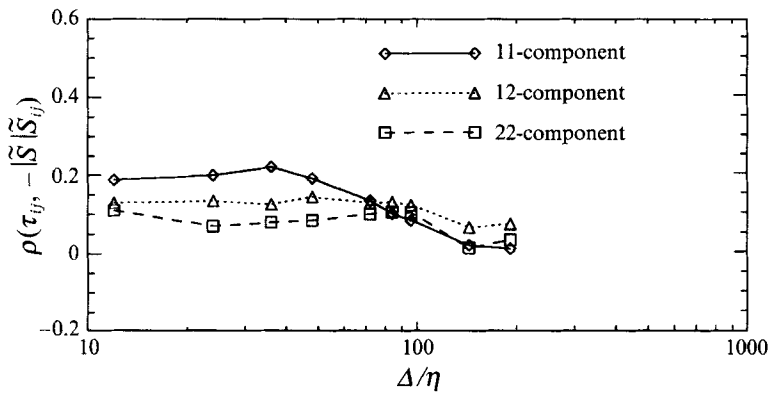
FIGURE 8. Correlation coefficients between elements of \tau_{ij} and -|\tilde{S}|\tilde{S}_{ij} as function of filter width \Delta (top-hat filter) for different tensor components.
