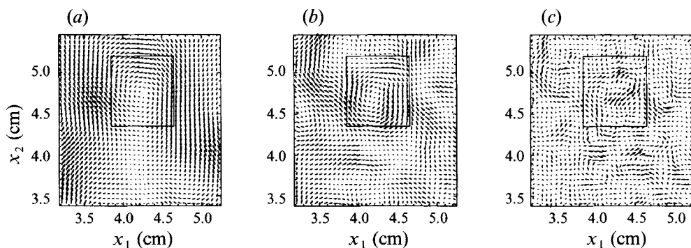
FIGURE 14. Velocity maps in consecutive bands, of characteristic scale L/2^n (where L = size of entire image). From (a)–(c): n = 3, 4, 5 . The bands are defined as the difference between two low-pass-filtered versions of the velocity field. Larger-scale fields are sampled on coarser grids that properly emulate the information available during LES. Bilinear interpolation is used to generate smooth fields, for graphical purposes. To avoid crowding, only a subset of an image is shown. Some similar features in vortical regions can be recognized in consecutive bands.
