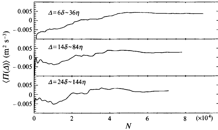
FIGURE 10. Running average ( \sum_N \langle \Pi \rangle / N ) of the SGS energy flux as function of number of data points N employed to compute the average. The top-hat filter is used.
