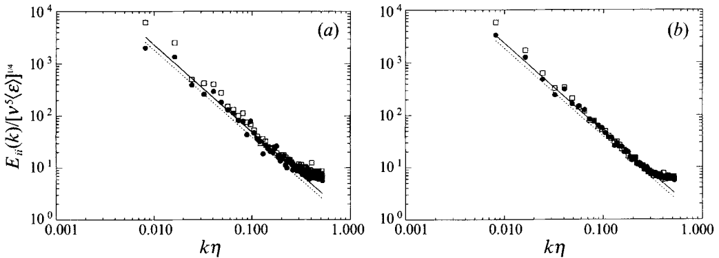
FIGURE 4. (a) Radial two-dimensional energy spectrum in Kolmogorov units, of the vector field shown in figure 2. Circles and squares are for the u_1 and u_2 components, respectively. Lines show the Kolmogorov spectrum (without a dissipation range), for C_k = 1.6 (dotted line) and C_k = 2 (solid line). (b) Same as (a), but averaged over all six images.
