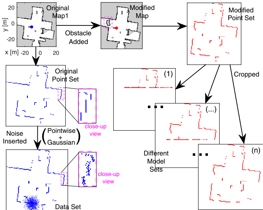
Figure 2. Synthetic laser scan data generation for similarity rate definition performance tests.
