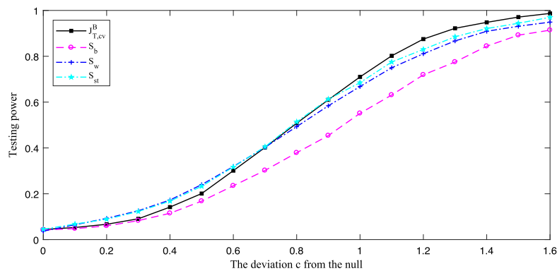
FIGURE 2. The testing power curves of the tests under DGPP.2.
