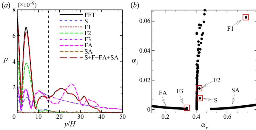
Figure 22. (a) Case 1 FFT amplitude of disturbance pressure and its projection on discrete modes S and F and continuous branches SA and FA, and (b) eigenvalue spectrum at x/H = 1432 for F = 2.822 \times 10^{-4} and \beta = 0 . The vertical dashed line marks the boundary-layer edge.
