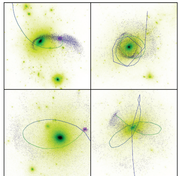
Figure 2 Some sample orbits of satellite galaxies within our set of dark matter host halos. We can clearly see how well we trace the orbits and follow the tidal disruption of the satellites, respectively.
