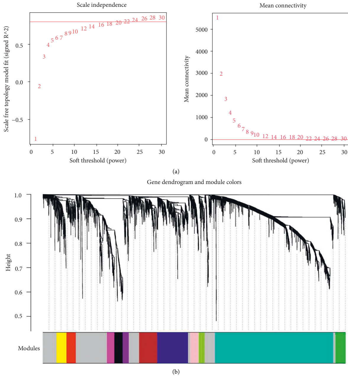
FIGURE 4: As shown in Figure 4(a), we select the value of power when the square value of correlation coefficient reaches 0.9 for the first time, that is, power = 22. As shown in Figure 4(b), a total of 12 modules are obtained.
