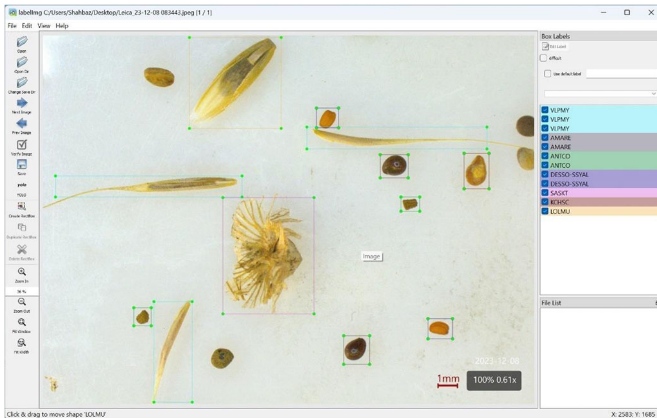
Figure 1. labelmg-generated bounding boxes drawn around weed seeds belonging to different classes. Each colored box and number corresponds to a distinct class of weeds. Bounding boxes aid in identifying and localizing weed seeds within images, assisting in the accurate classification and detection of various weed species. Understanding the representation of bounding boxes is fundamental for interpreting object detection results.
