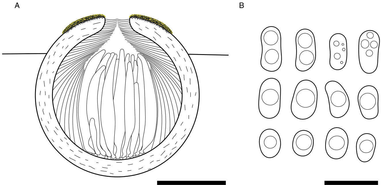
Figure 2. Thelocarpon periphysatum . A, schematic section of a perithecium; the periphysoids are more appressed to the exciple than appears in the drawing. B, ascospores. Scales: A = 100 \mu\text{m} ; B = 10 \mu\text{m} . In colour online.
