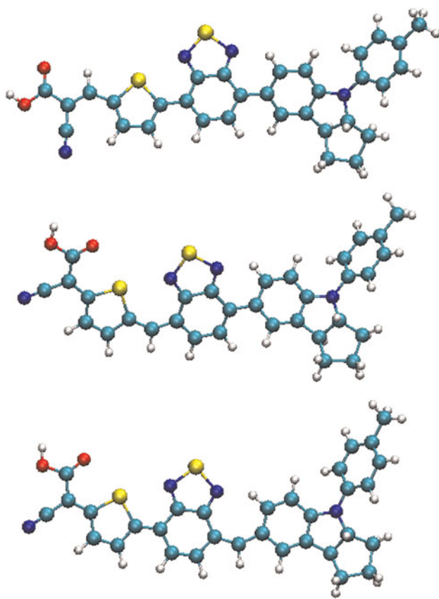
Figure 1. The structures of the dyes (top to bottom) WS-2, WS-2.1, and WS-2.2. Atom color scheme: C—cyan, S—yellow, N—blue, O—red, H—grey.
