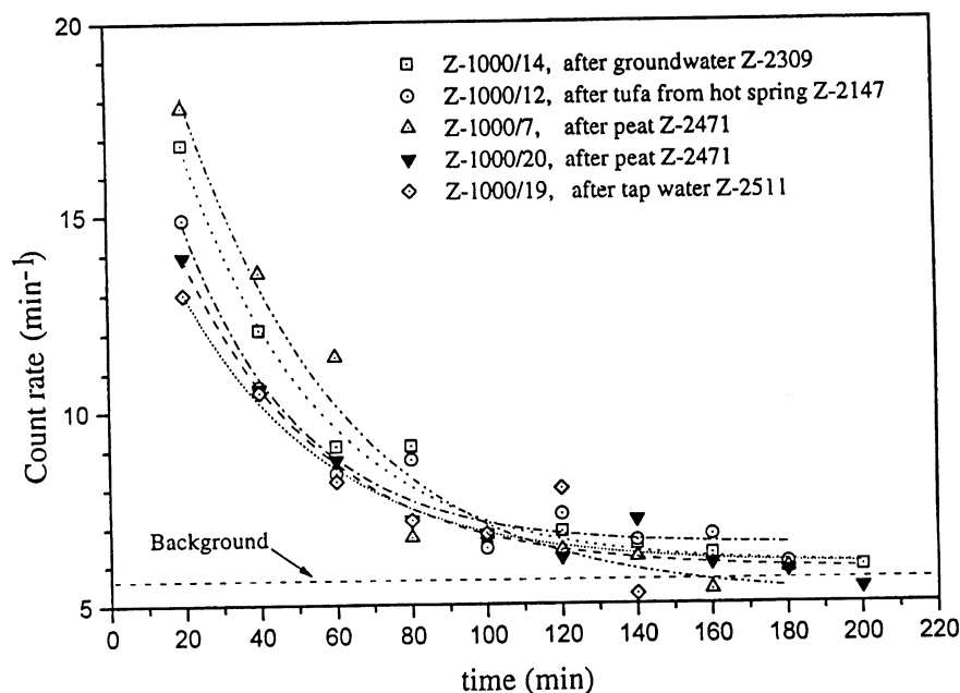
Fig. 4. The decrease of the background count rate after replacing the Rn-contaminated samples with background samples. The exponential functions fitted to the data points correspond to the decay curve of ^{214}\text{Pb} with an average half-life of 26 min.
