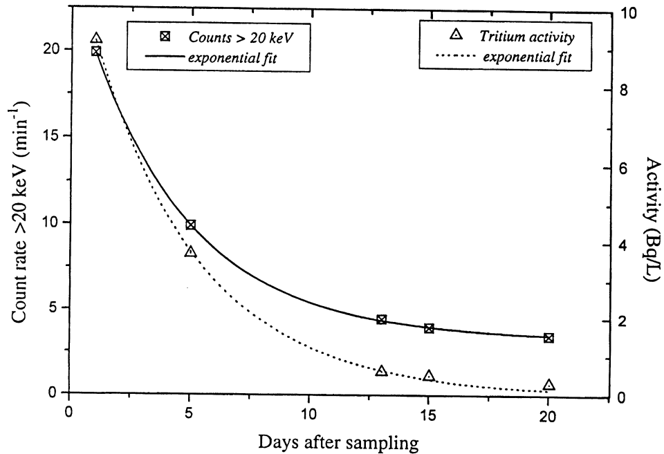
Fig. 6. Apparent ^3\text{H} activity measured in ^3\text{H} energy window (1–10 keV, right scale) and the count rate in the energy window above 20 keV (left scale) in groundwater sample (T-1583) as a function of the number of days after sample collection. Excess count rates in both windows indicated ^{222}\text{Rn} as the source of contamination.
