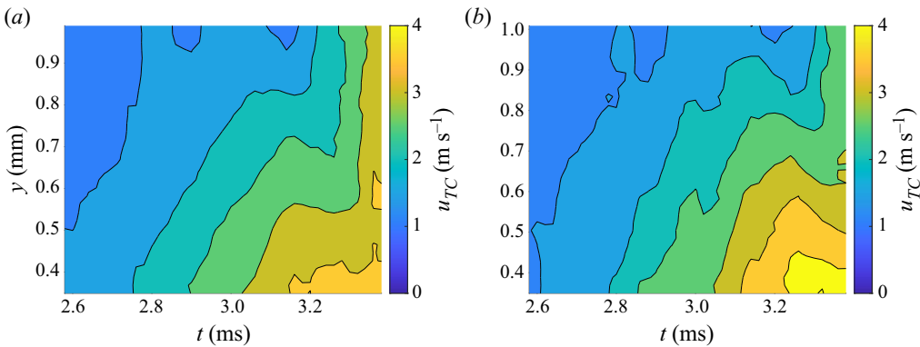
Figure 7. Measured rim velocity to the left and right side of the corona centreline. Impact parameters: D_0 = 2 mm, U_0 = 3.2 m s -1 , H_{f0} = 80 \mu m. The velocities on both sides are shown as positive values for better comparison.
