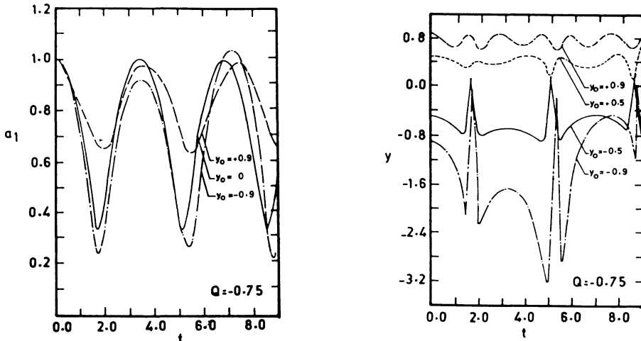
Figure 1. a) Behavior of the a_1 -axis with time for Q = -0.75 and for various values of initial eccentricities y_0 . b) Behavior of the eccentricity with time for Q = -0.75 . The ordinate y measures the eccentricity; it is positive (negative) for oblate (prolate) spheroids.
